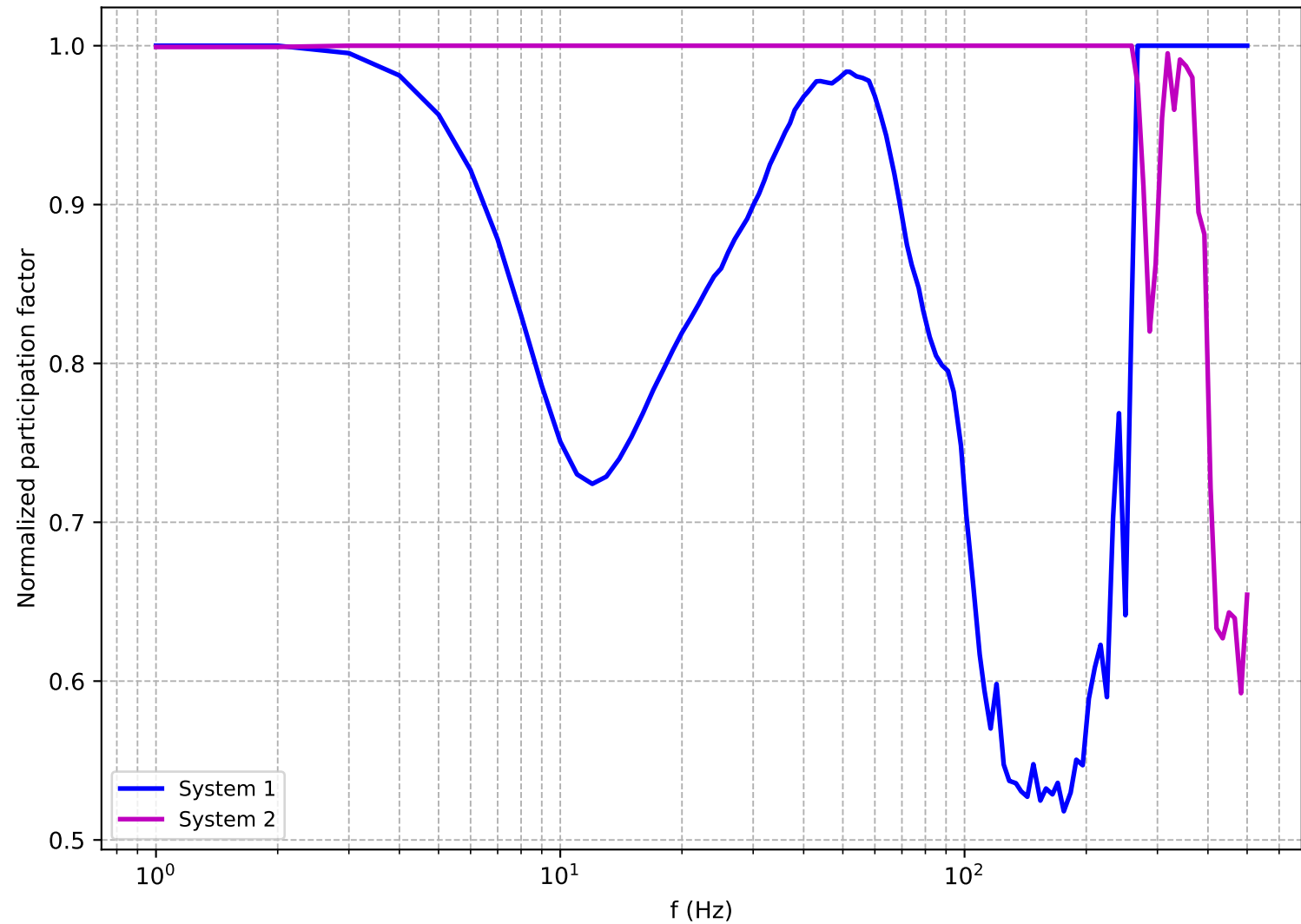
Participation factors of critical mode vs frequency
